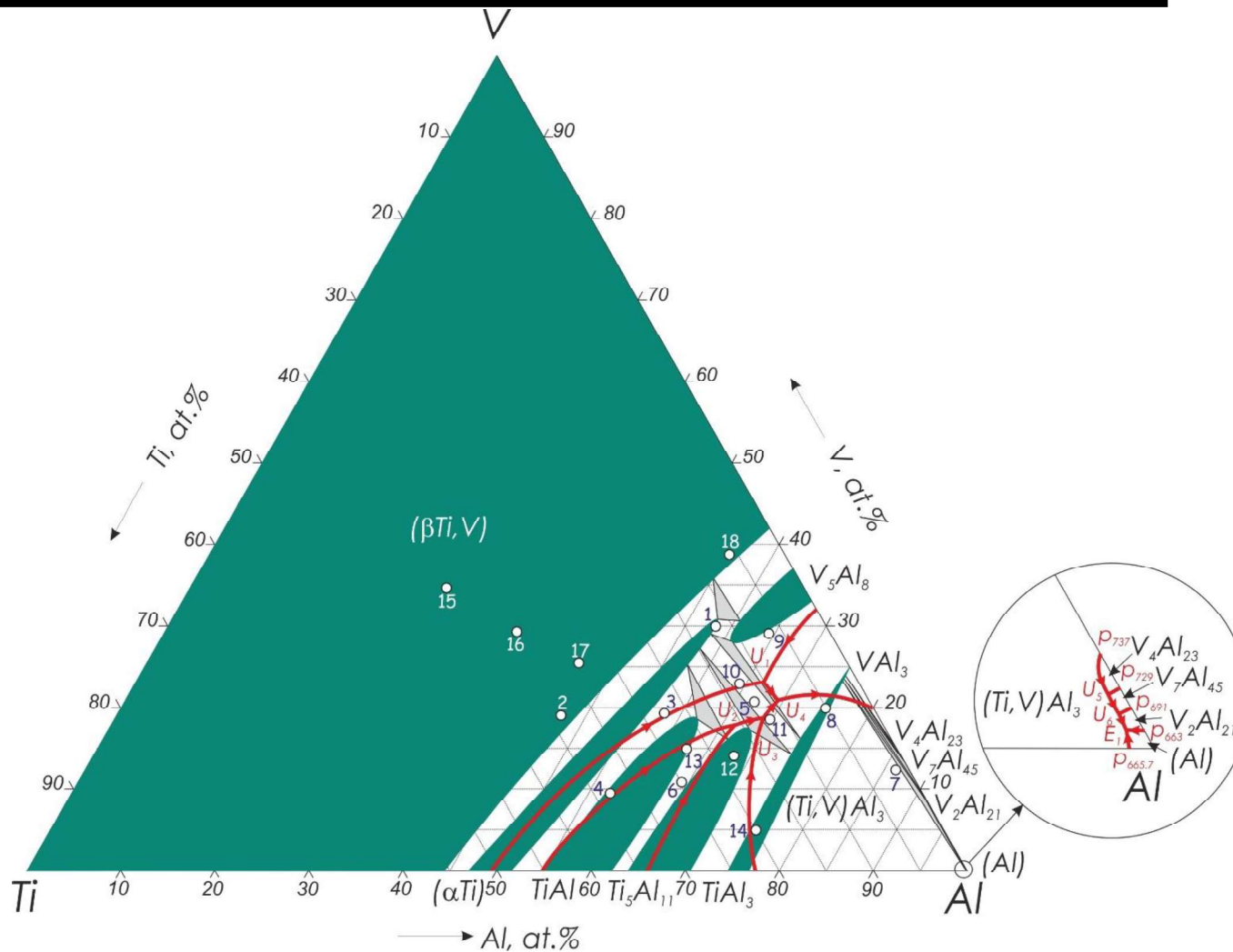
Fig. 1. Liquidus and solidus projections of the Al-Ti-V system:
